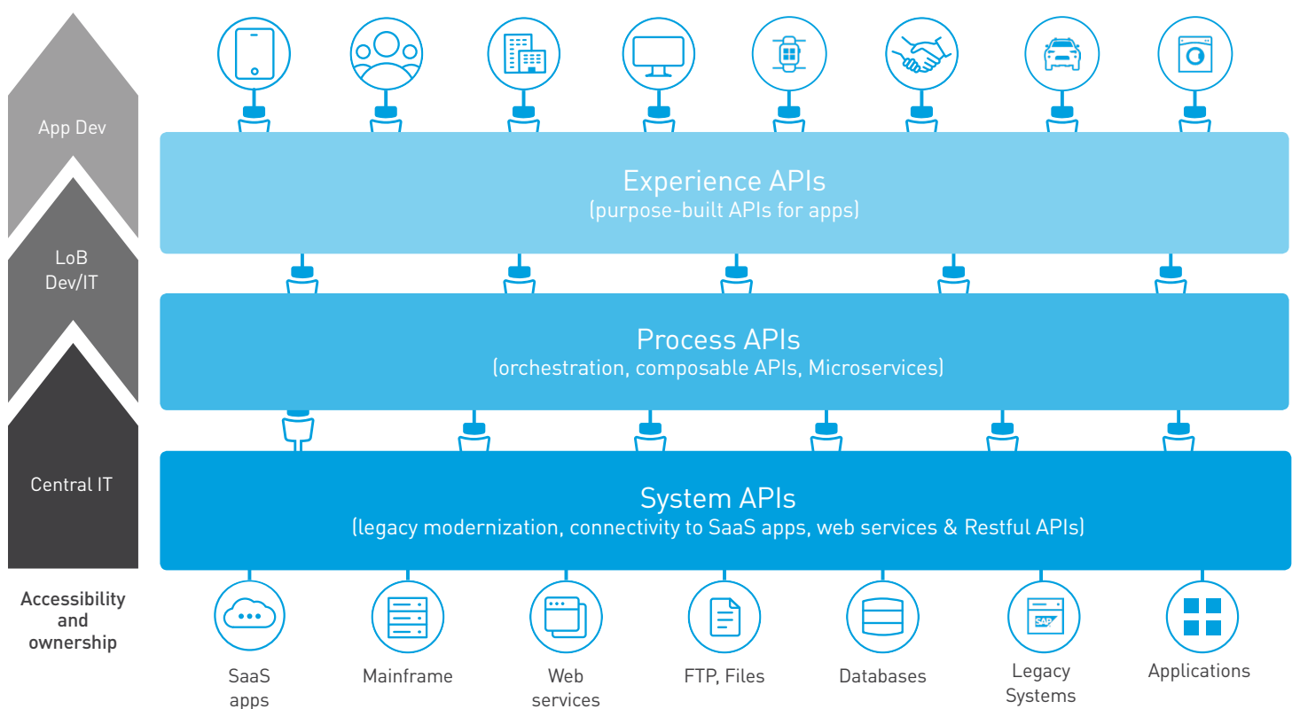
Figure 1: Microservices classification
